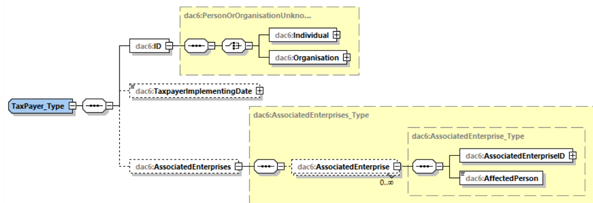
Figure 6: DAC6 Relevant Taxpayer Diagram
