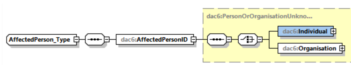
Figure 14: DAC6 Affected Person Type Diagram
