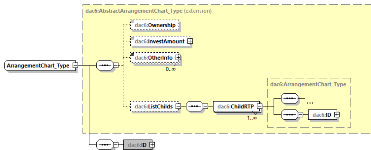
Figure 19: DAC6 Arrangement Chart Type Diagram
